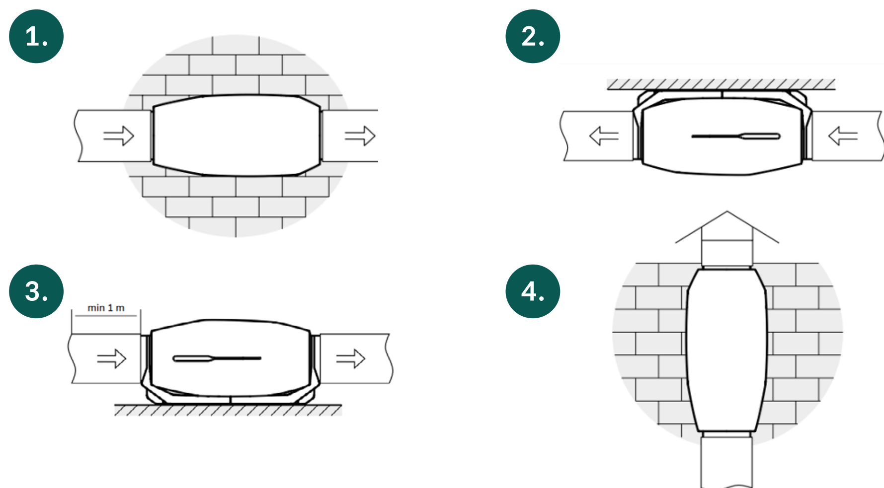
1. Horizontal wall mounting | 2. Ceiling mounting | 3. Mounting on the floor | 4. Vertical wall mounting
